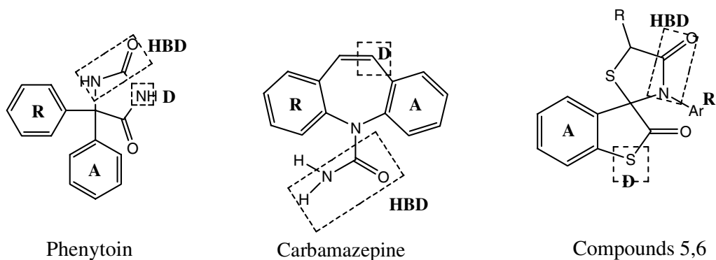
Fig. 1: Anticonvulsant agents showing the required pharmacophoric elements
