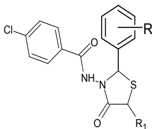
Scheme 8: R1=H, CH 3 , CH 2 COOH, R=H, 2-NO 2 , 4-NO 2 , 4-OCH 3 , 3, 4-(OCH 3 ) 2
