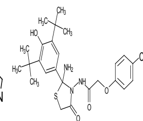
Scheme 23
