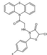
Scheme 12
