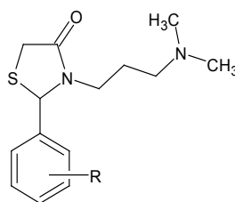
Scheme 18: R=3-CONH 2 , 3-CHO, 3-CHNOH
