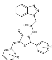
Scheme 13: R=Cl, CH 3 , NO 2 , Br
