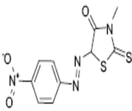
Scheme 28
