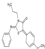
Scheme 14
