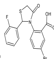
Scheme 15
