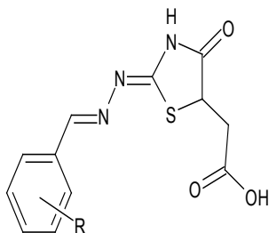
Scheme 4: R = 2-fluoro, 4-fluoro, 4-dimethylamino, 2,4-dimethoxy, 2,4-dichloro, 3,5-di-tert-butyl-4-hydroxy
