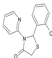
Scheme 10
