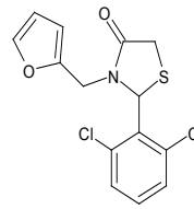
Scheme 11
