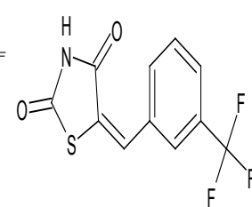
Scheme 21
