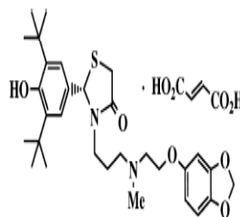
Scheme 16
