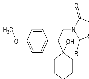
Scheme 3: R = 4-hydroxyphenyl, 4-methylphenyl, 2-nitrophenyl R = 4-methoxyphenyl, 2-butyl-4-chloro-imidazole-5-yl
