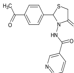
Scheme 24
