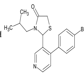
Scheme 17
