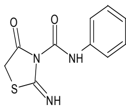
Scheme 29
