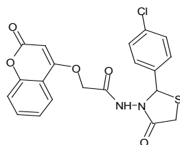
Scheme 26
