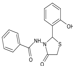
Scheme 27
