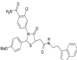
Scheme 32
