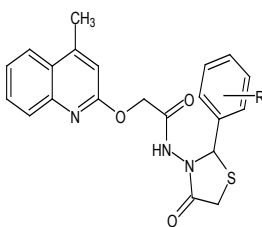
Scheme 30
