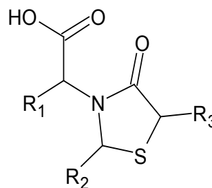
Scheme 5: 2,3,5 Trisubstituted -4-thiazolidinone
