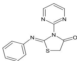
Scheme 25
