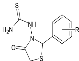
Scheme 31: R=4-N(CH 3 ) 2 , 4-OCH 3
