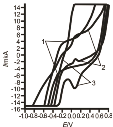
Fig. 2: Cyclic voltammograms GSH at: GE (1), AuNP-GCE (2), Au-GE (3) in solution 0,1 M NaOH, C_{GSH} = 1,3 \cdot 10^{-12} M; scan rate 100 mV·s -1
