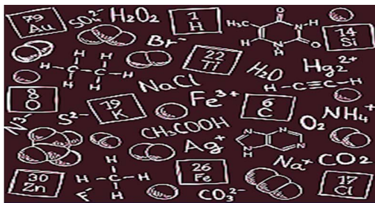
Fig. 3. Some chemical elements formula expression
