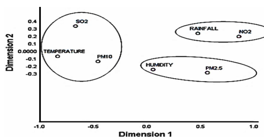
Fig. 3. MDS graph of summer season
