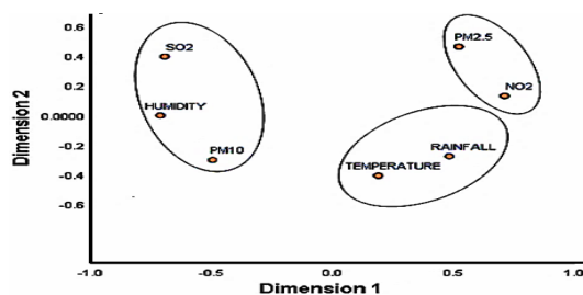
Fig. 4. MDS graph of Rainy season
