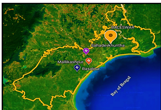
Fig. 2. Sampling stations in Baleswar District
