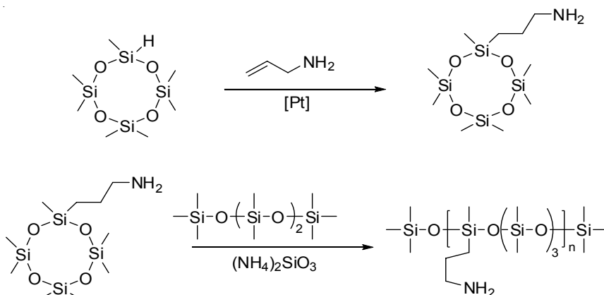
Fig. 9. Functionalization of cyclosiloxane by hydrosilylation and ring-opening polymerization
