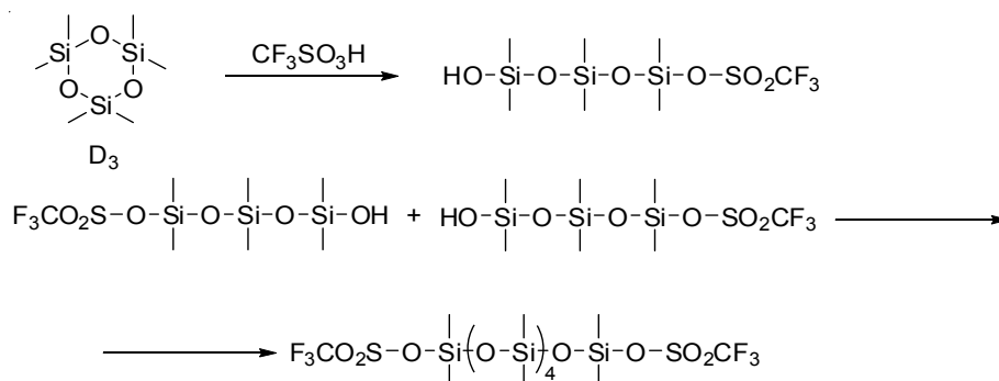
Fig. 1. Synthesis of low molecular weight POS by the cationic polymerization method with ring opening
