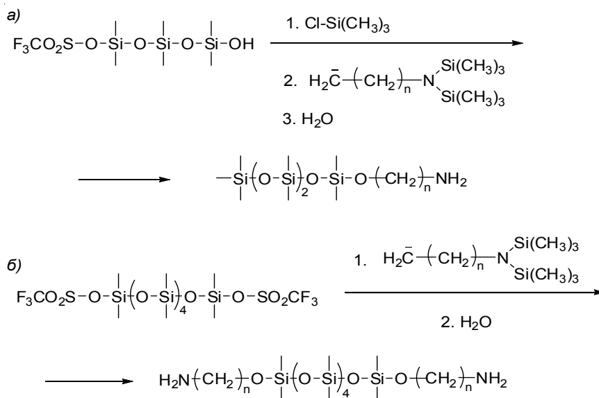
Fig. 2. Methods for the modification of oligomers prepared by the acidolysis condensation of cyclosiloxane
