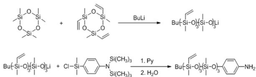
Fig. 7. Anionic copolymerization of two cyclosiloxanes
