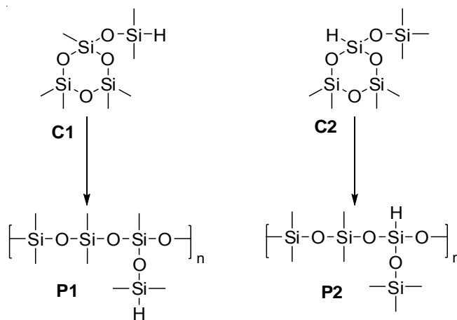
Fig. 3. Preparation of POS of a various structures by an anionic ring-opening polymerization
