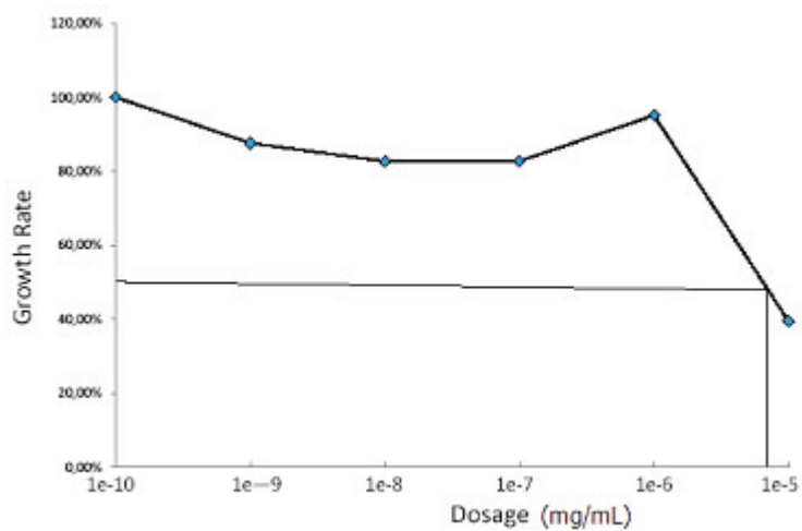
Fig. 3: In vitro antiplasmodial assay of artonin E (2)
