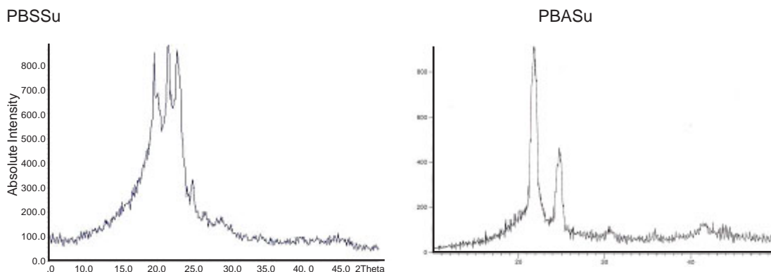
Fig. 3: WAXD diffractogram of polyesters
