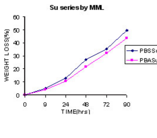
Fig. 5: Biodegradation analysis of polyesters using Mucor miehei lipase enzyme
