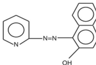
Scheme 1: Synthesis and Molecular structure of Schiff's Naphtol-2-(Pyridylazo-2)-1 (PAN)
