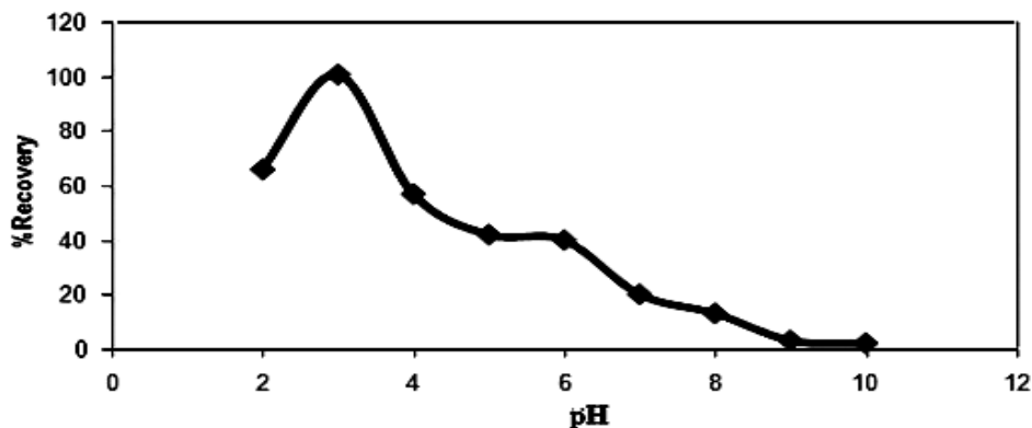
Fig. 1: Extraction percentage of Cu(II) against pH
