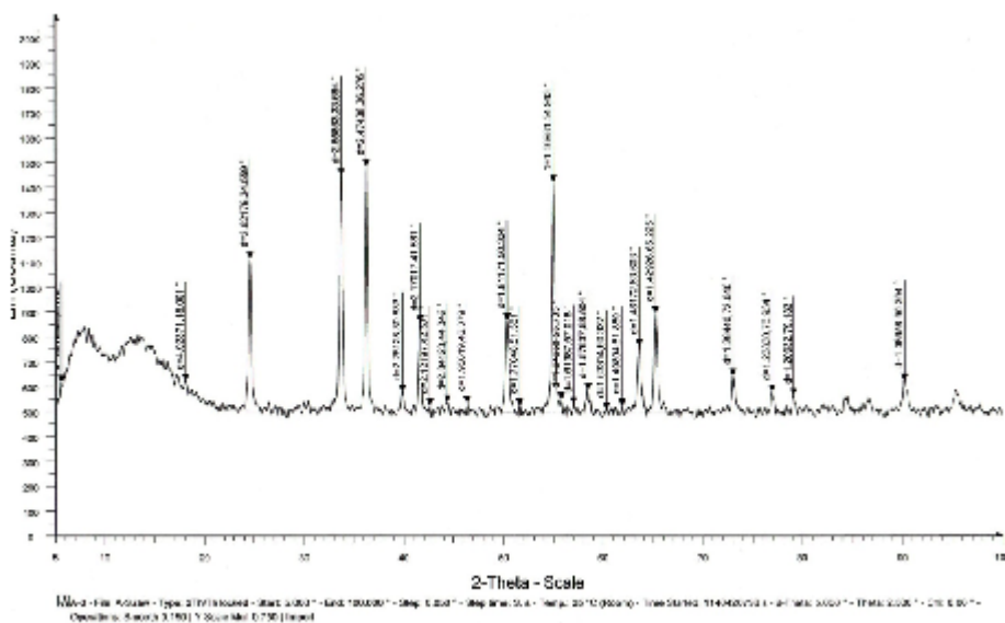
Fig. 1: X-ray diffraction for chromium oxide ( \text{Cr}_2\text{O}_3 )
