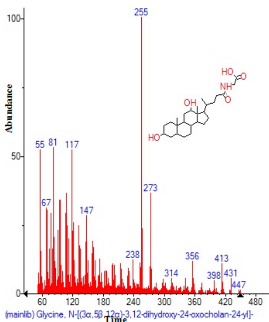
Fig. 28: Structure of Glycine ,N-[(3α,5β,12α)-3,12-dihydroxy-24-oxocholan-24-yl] with RT: 28.893 present in Cassia fistula
